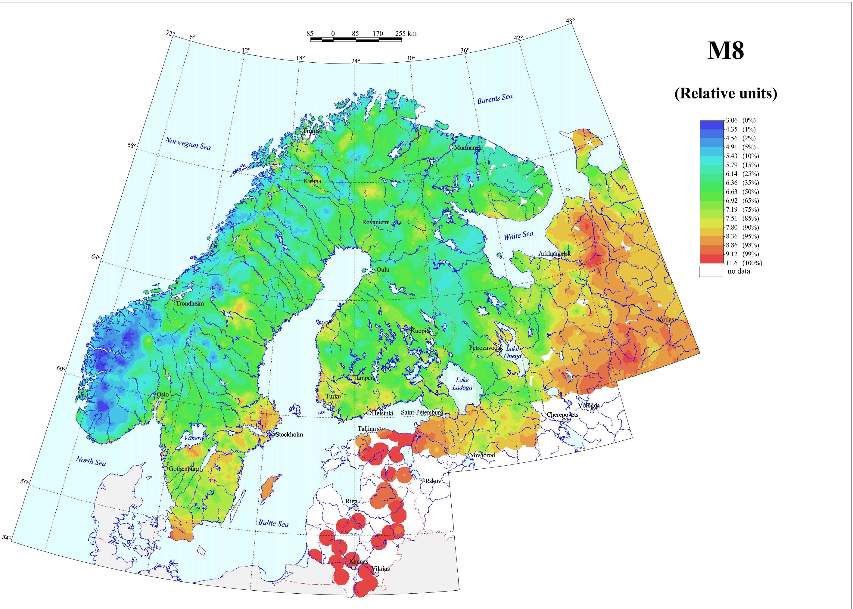
M8 (Ca, Mg) in Surface Water
